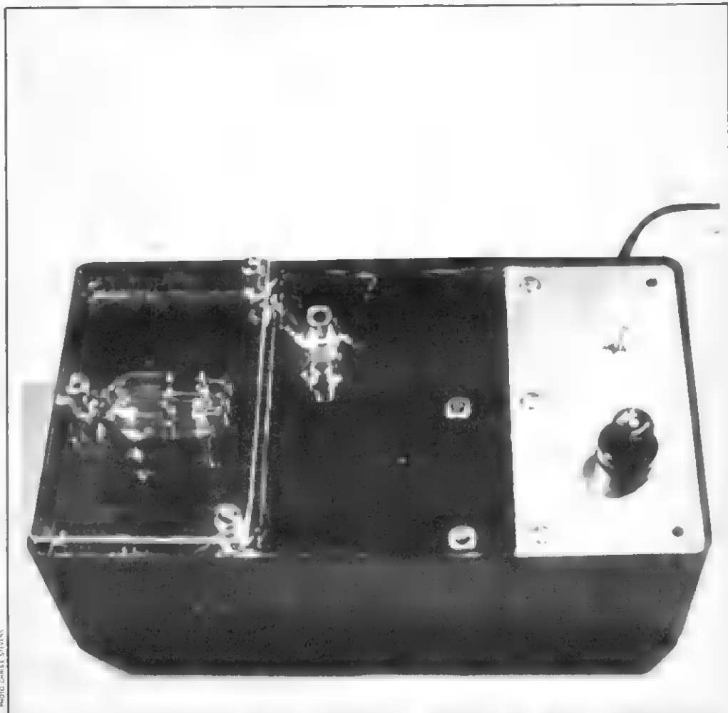
Opposite page: top view of the completed sync strobe circuit with all the parts in place. You can use this photo as a parts placement reference. Make sure parts are properly installed before plugging unit in. Above: the completed project, the acrylic plastic safety shield covering the strobe tube.
